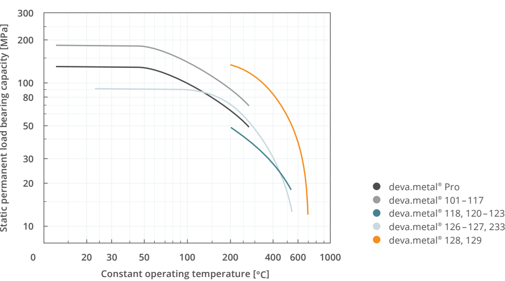
Temperature influence on the static permanent load bearing capacity of deva.metal®
