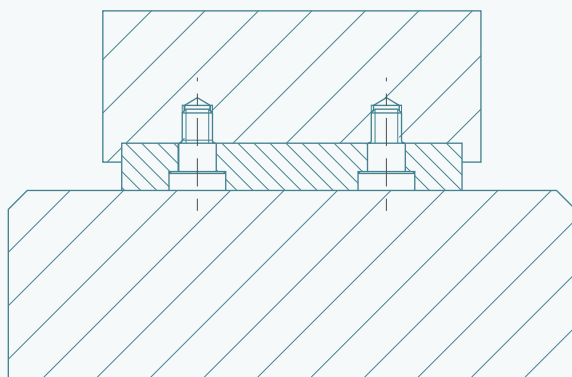
DEVA® special screw after assembly
